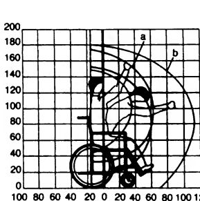
⑩ Side elevation
